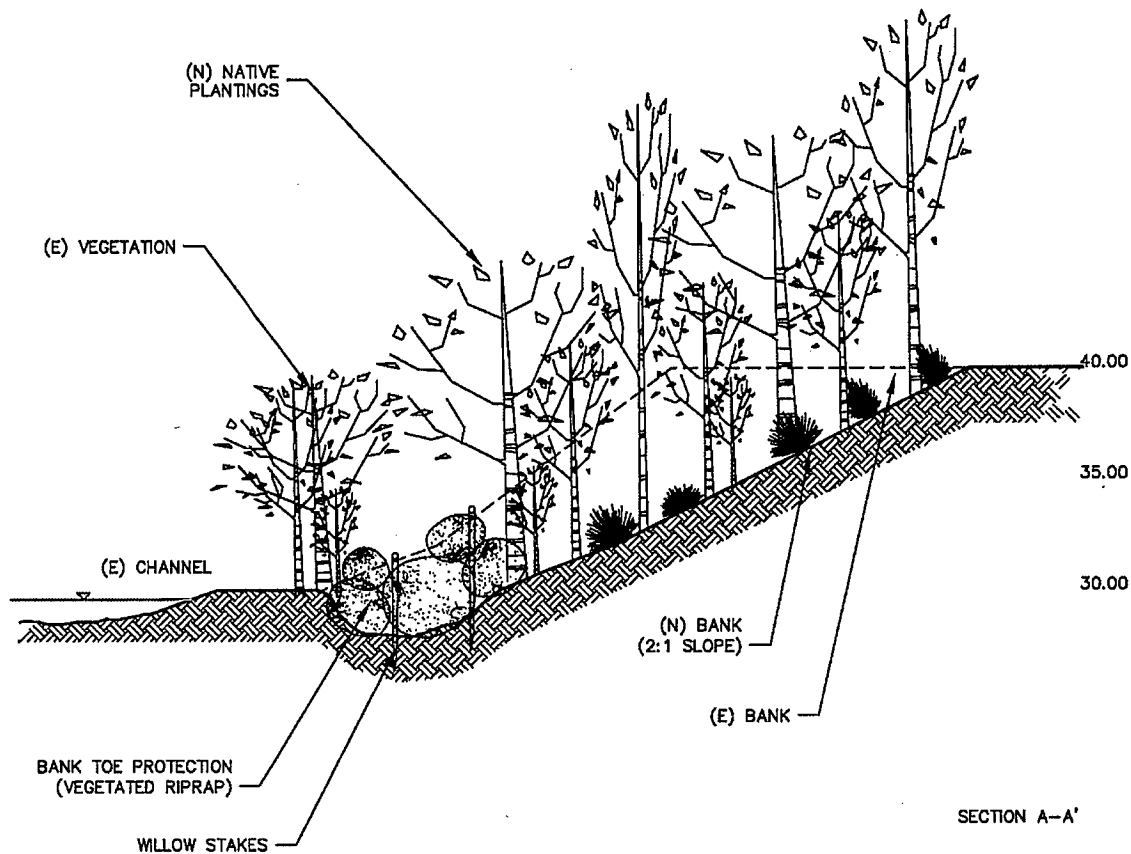
Figure 4. Andrew Molera Conceptual Project Design
