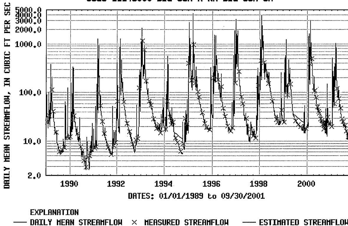
Figure 5. Measured Daily Mean Flows at USGS Big Sur gage 1989-2002
